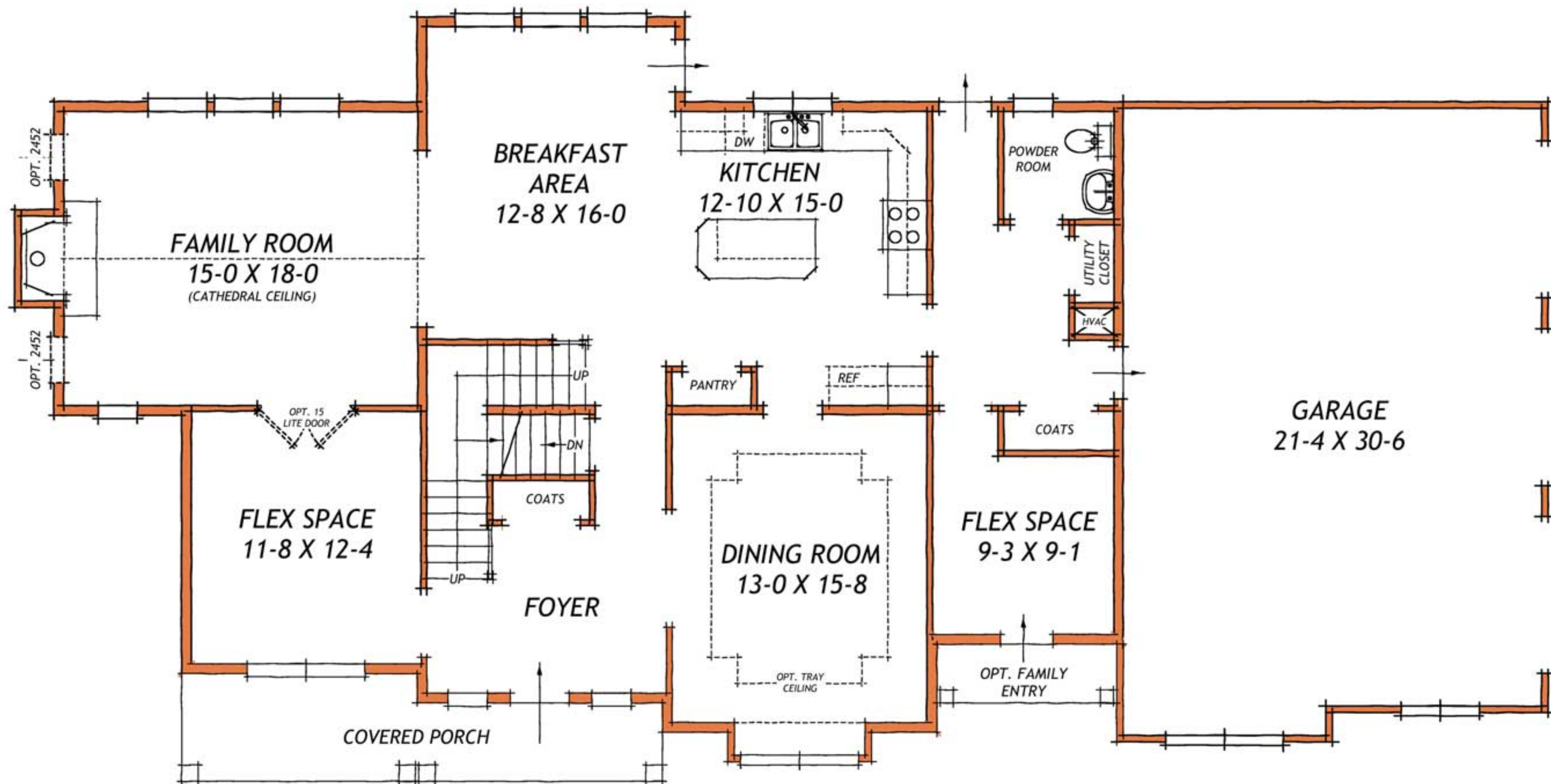
FIRST FLOOR PLAN "C"
